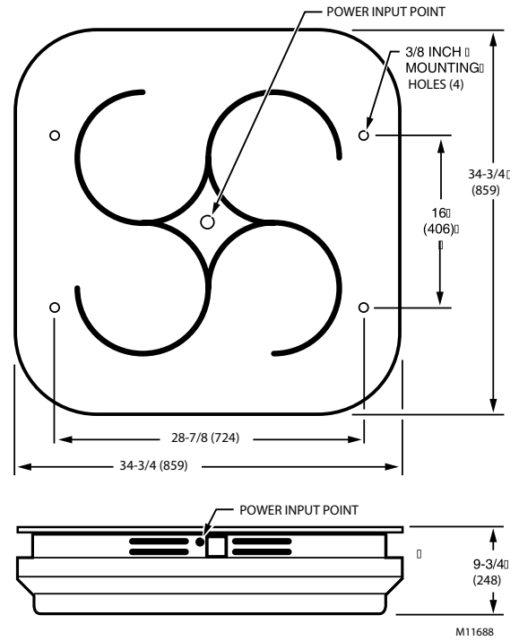
Fig 1. CA115 dimensions in in. (mm).
