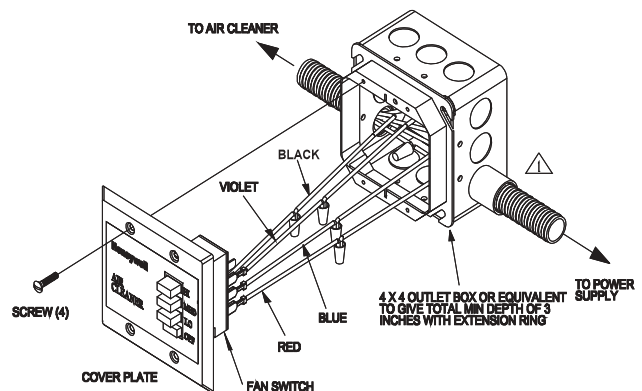
Fig. 6. Wiring 3-Speed Remote Switch
