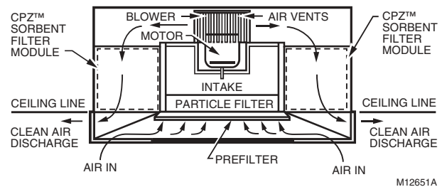
Fig. 8. CA111 (series 1,2,3) air cleaner operation.
