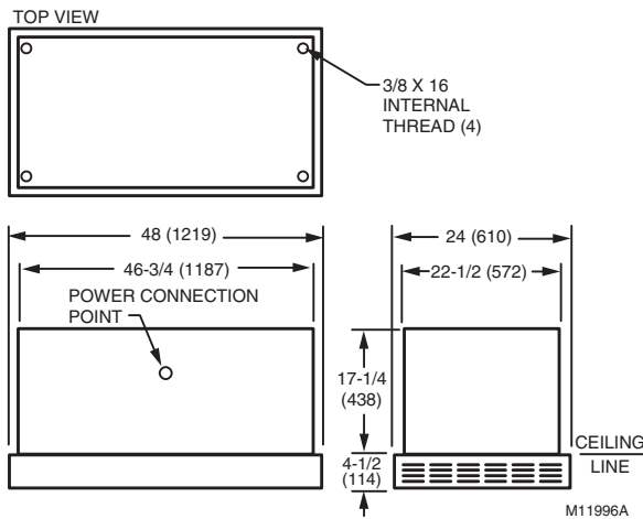
Fig. 1. Approximate dimensions of CA111 (Series 1,2,3) in in. (mm).
