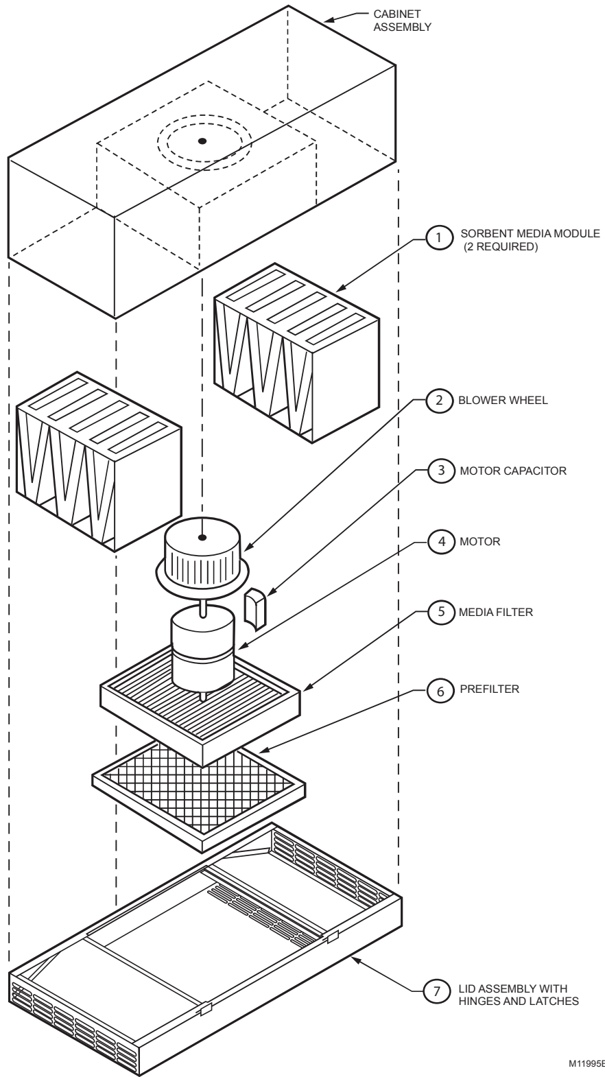
Fig. 9. Exploded view of CA111 (series 1,2,3) in Ceiling Media Air Cleaner components.
