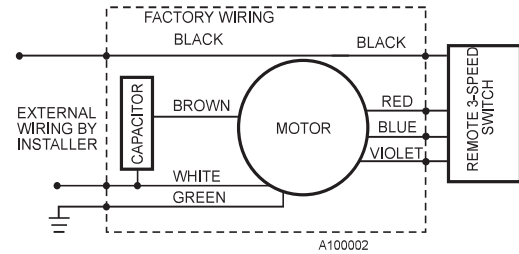
Fig. 4. Typical CA111 Series 3 only 120V, 60 Hz or 230V, 50 Hz wiring diagram.
