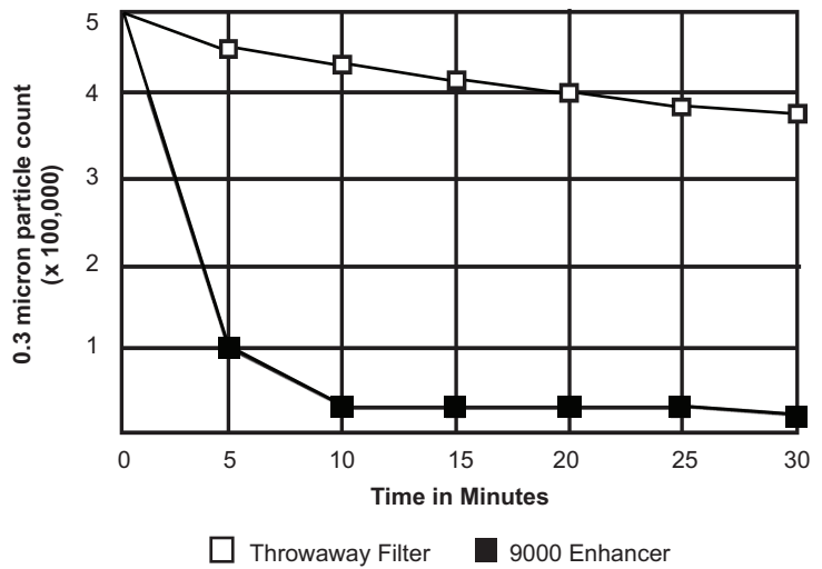
Performance Comparison Test Casino Air 9000 Enhancer vs. Disposable Particulate Filter
