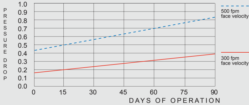
PRESSURE DROP LIFE CYCLE PERFORMANCE FOR A MODEL CA7000 BASED ON CONSTANT AIR VOLUME SYSTEM
