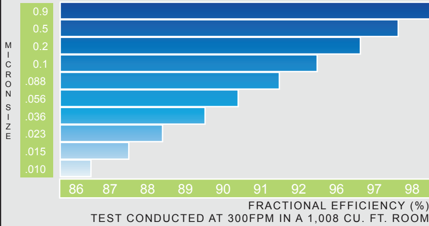
MODEL CA7000 FILTRATION PERFORMANCE OVER 30 MINUTES OF CONTINUOUS OPERATION (AS PER AHAM STANDARDS)
